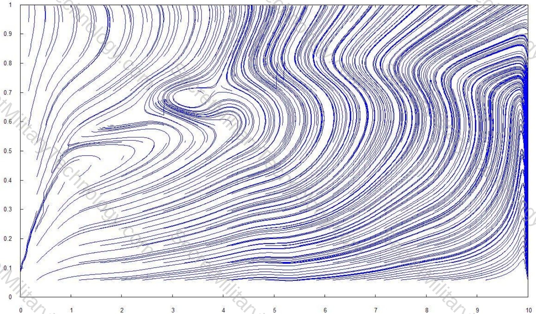
NIMROD MHD Simulation: Step 450000 = 425 \mu s
