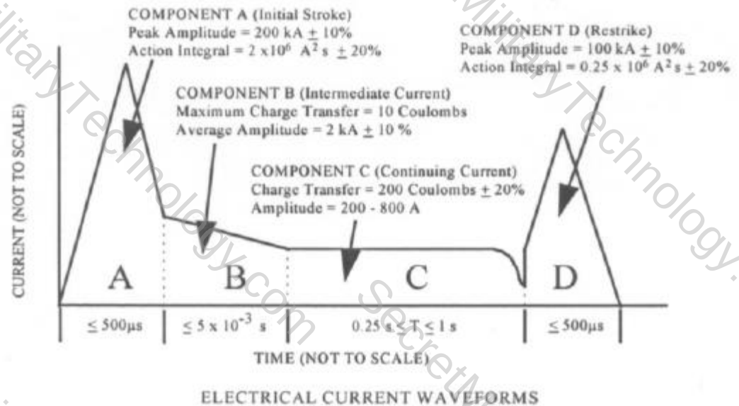
Idealized lightning current waveform
